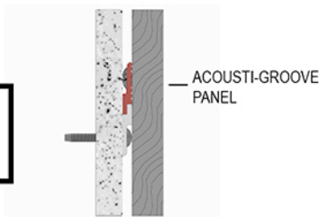
Z-Clip
